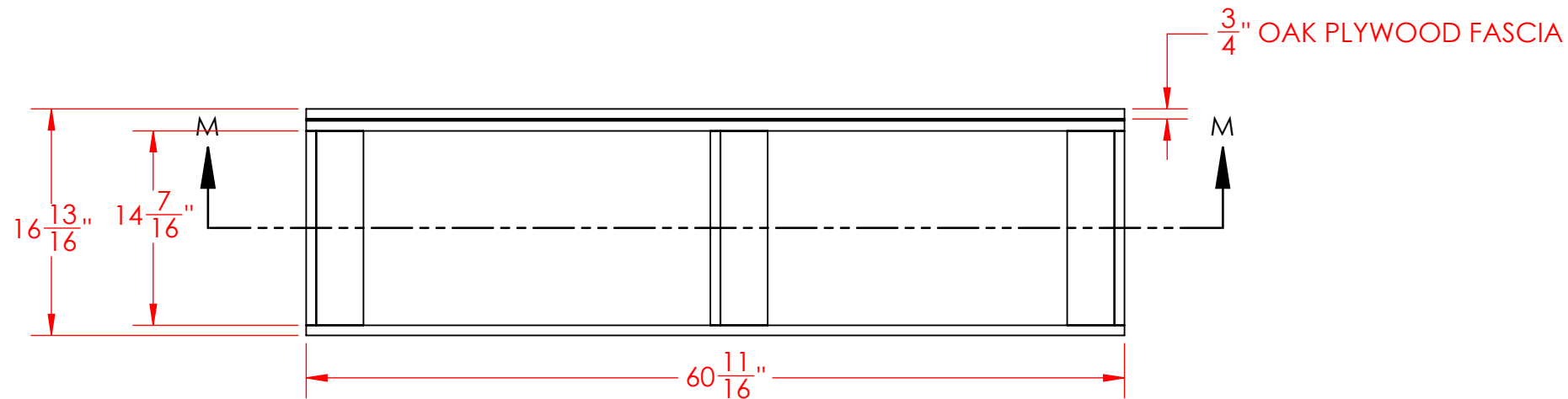
1 FW-03 BASE / TOP VIEW SCALE 1:12
