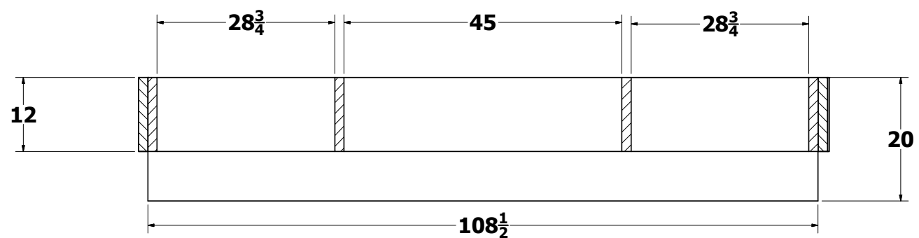
Front View SCALE 0.03 : 0.3
