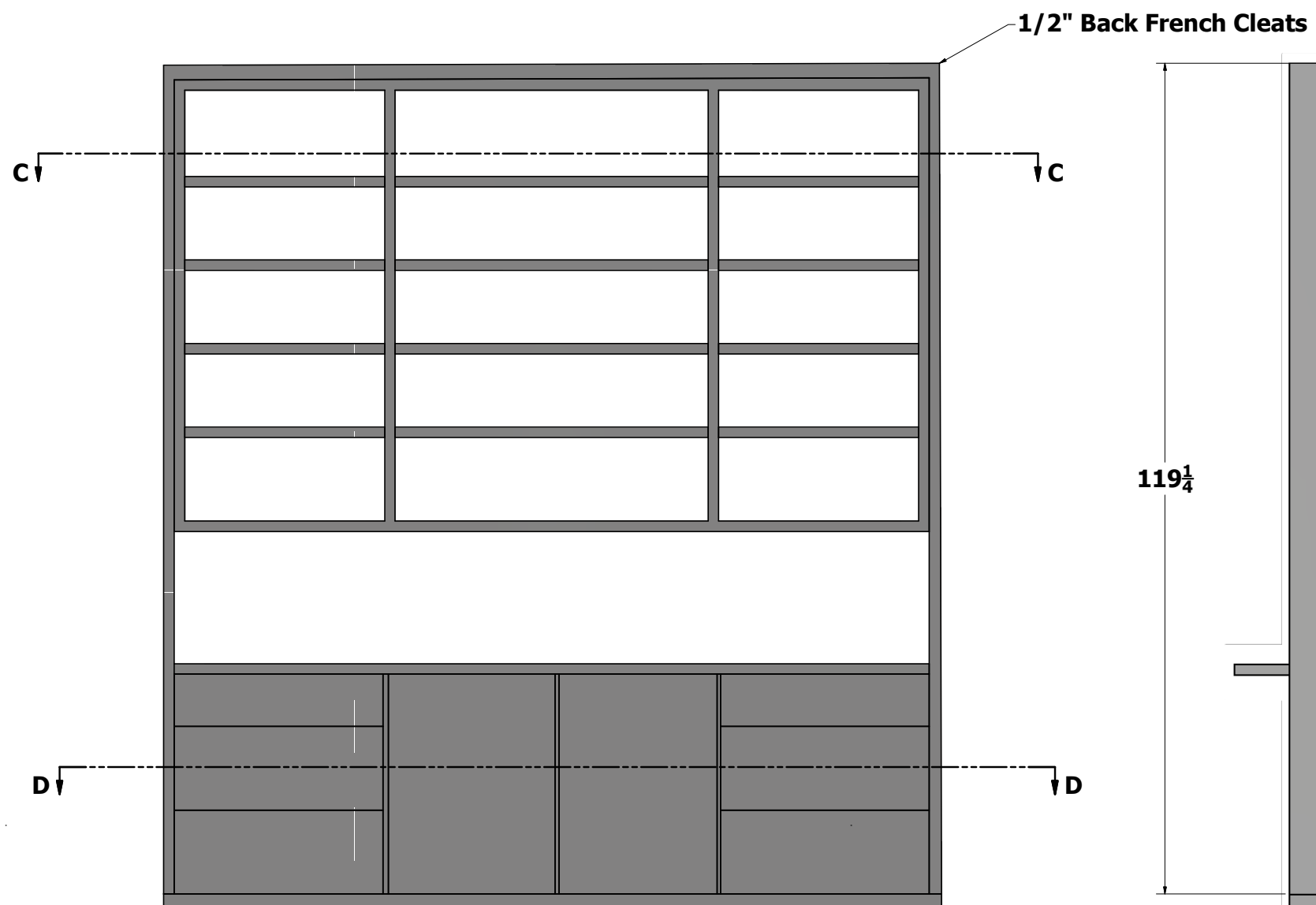
Front View SCALE 0.03 : 0.3
